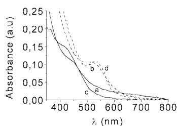
Figure 4. UV/Vis spectra of an aqueous solution of PDO-PEG (plot a) that was used as \text{Fe}^{3+} sensor and, therefore, transformed into TP-PEG (spectrum b, which was reused five times according to the cycle shown in Scheme 4 either in the PDO-PEG form (plot c) or after sensing with \text{Fe}^{3+} and transformation into TP-PEG (plot d).
