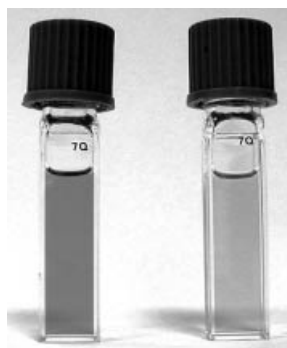
Figure 3. Photograph of two cells containing aqueous solutions of PDO-PEG ( 0.5 \text{ mg mL}^{-1} ) in the presence (left) or absence (right) of \text{Fe}(\text{NO}_3)_3 at a final concentration of 2 \times 10^{-4} \text{ M} .
