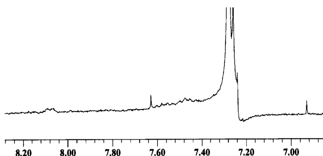
Figure 1. Expansions of part of the ^1\text{H} NMR spectrum of PDO-PEG.
