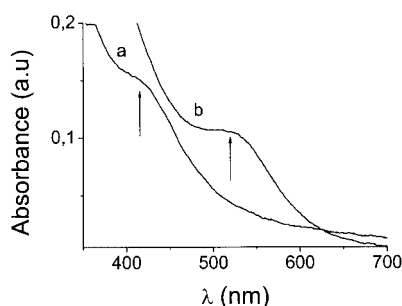
Figure 2. Transmission UV/Vis spectra of dichloromethane solutions of PDO-PEG (spectrum a) and TP-PEG (spectrum b). The arrows show the \lambda_{\text{max}} characteristic of PDO and TP precursors that are responsible for the color changes.
